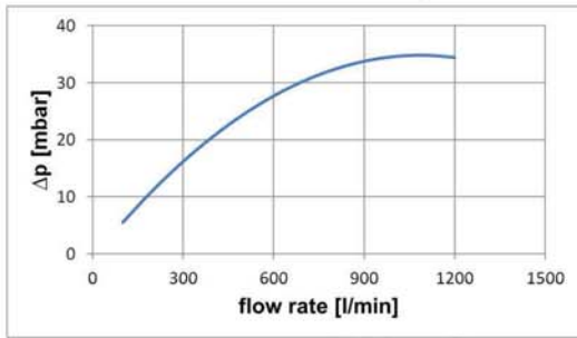
Pressure difference
